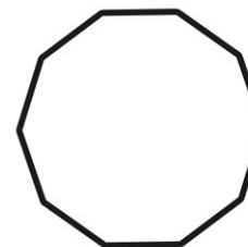
decagon
