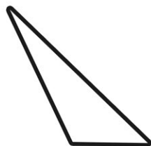
scalene triangle
