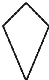
kite
