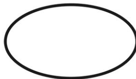
oval
